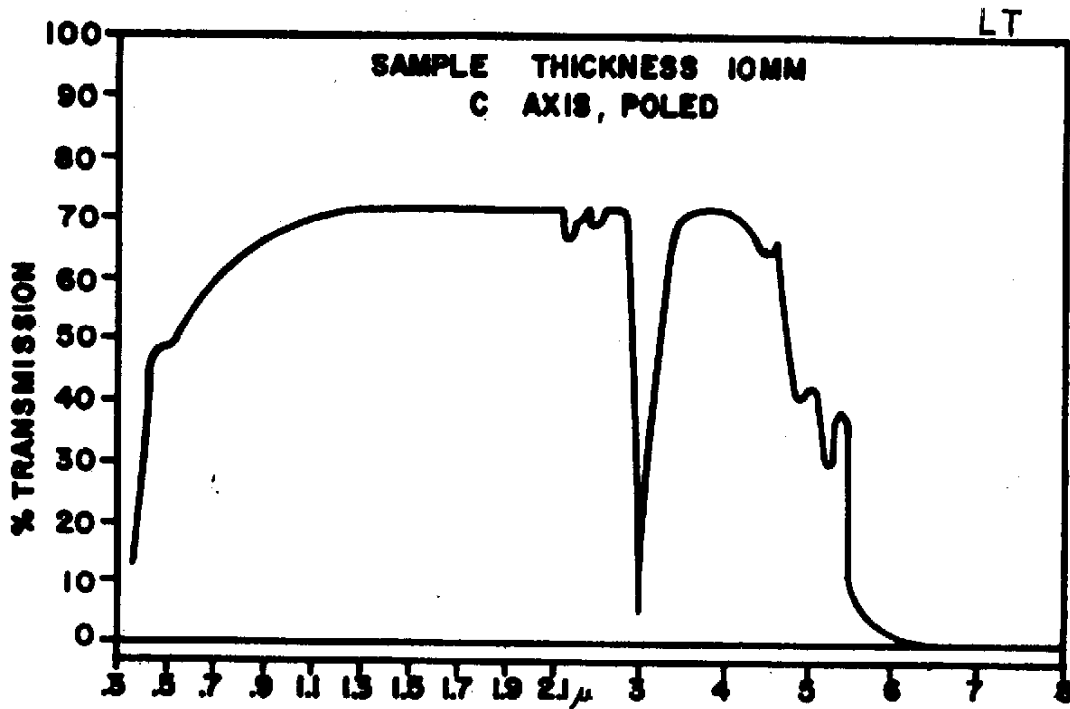
CURVE LITHIUM TANTALATE Percent transmission vs Wavelength
