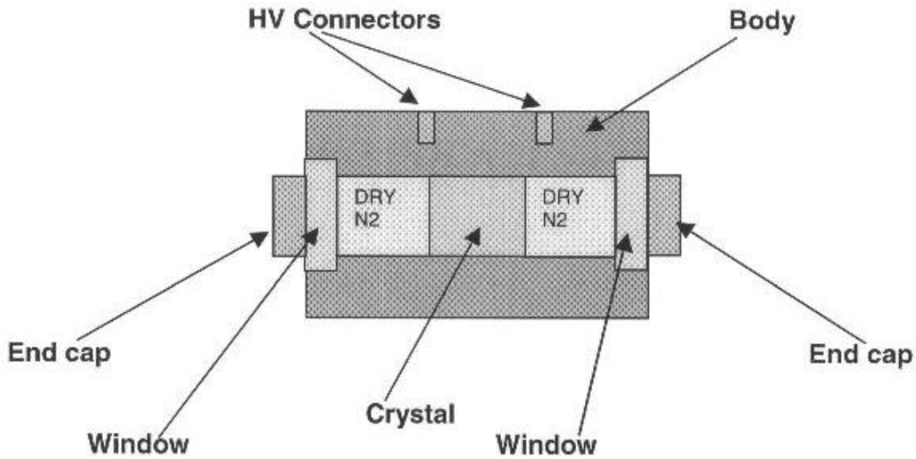
POCKELS CELL SKETCH
