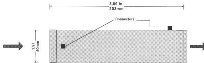
ELECTRO - OPTIC MODULATOR MODEL 22-50 Side view
